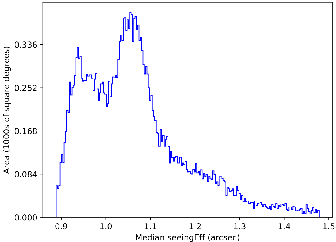
ddf_acor_sf20_lsf0_lsr0_v3.4_10yrs All sky all bands: Median seeingEff
