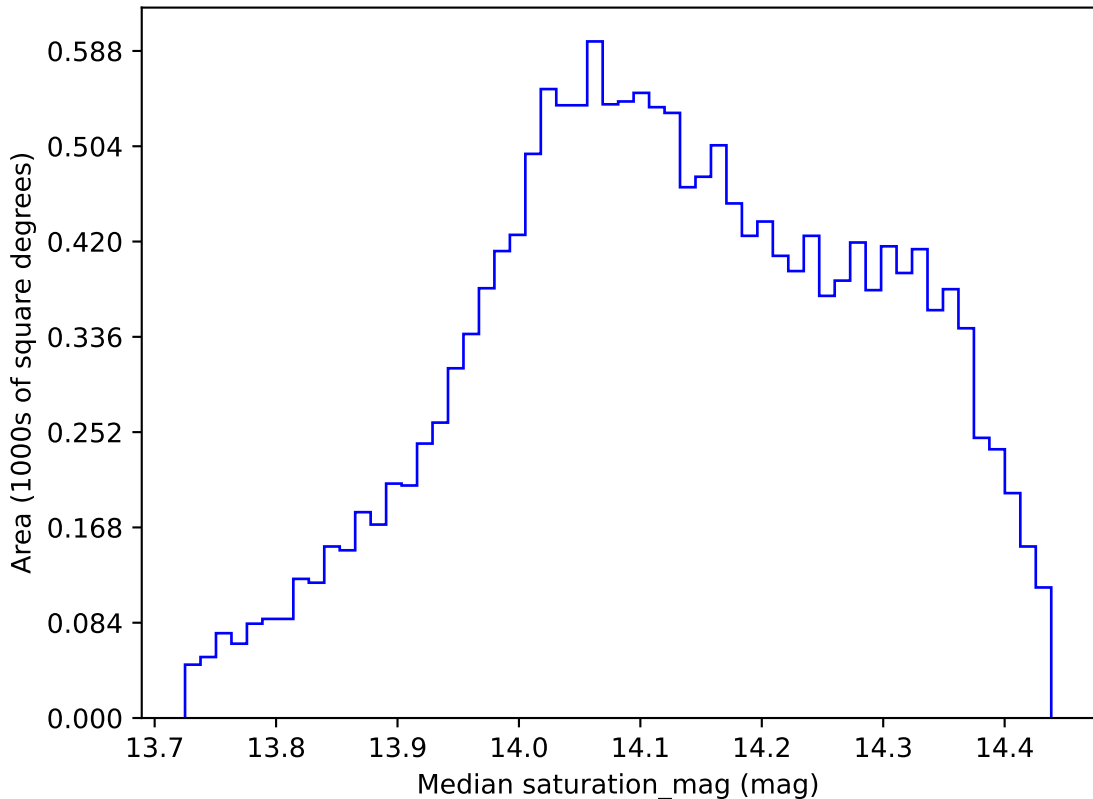
ddf_acor_sf20_lsf0_lsr0_v3.4_10yrs WFD z band: Median saturation_mag
