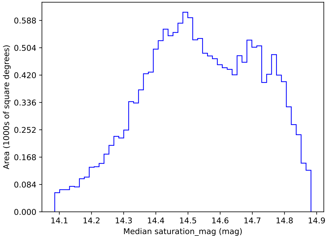
ddf_acor_sf20_lsf0_lsr0_v3.4_10yrs WFD i band: Median saturation_mag
