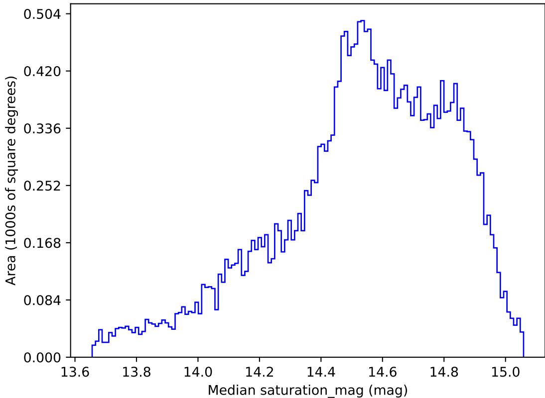
ddf_acor_sf20_lsf0_lsr0_v3.4_10yrs All sky r band: Median saturation_mag
