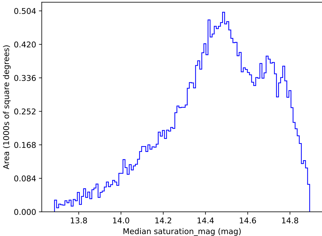
ddf_acor_sf20_lsf0_lsr0_v3.4_10yrs All sky i band: Median saturation_mag
