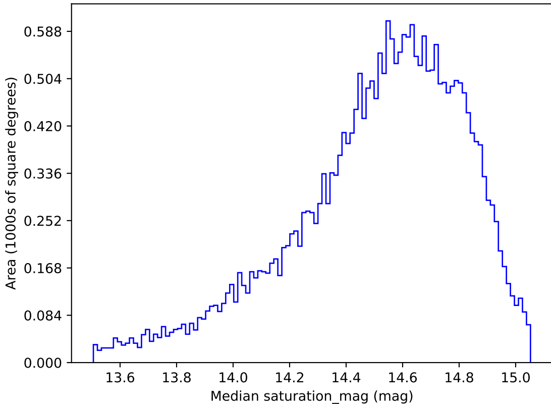
ddf_acor_sf20_ls0_lsr0_v3.4_10yrs All sky g band: Median saturation_mag
