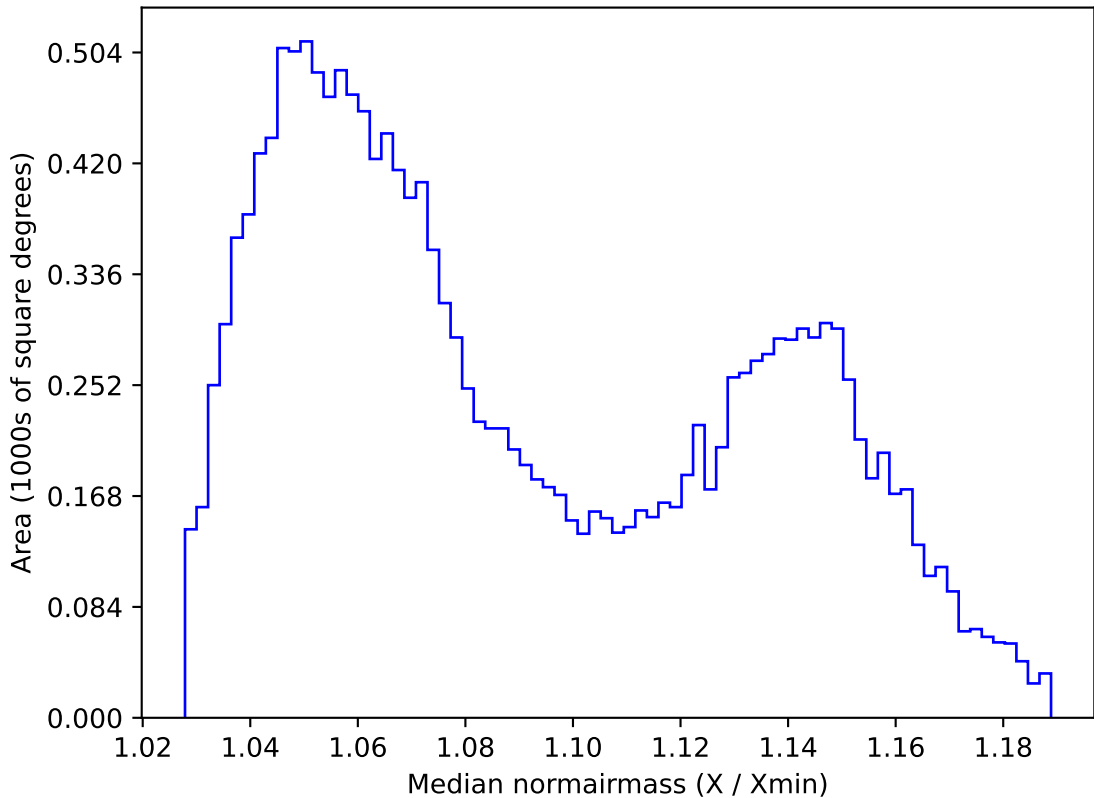
ddf_acor_sf20_lsf0_lsr0_v3.4_10yrs WFD y band: Median normairmass
