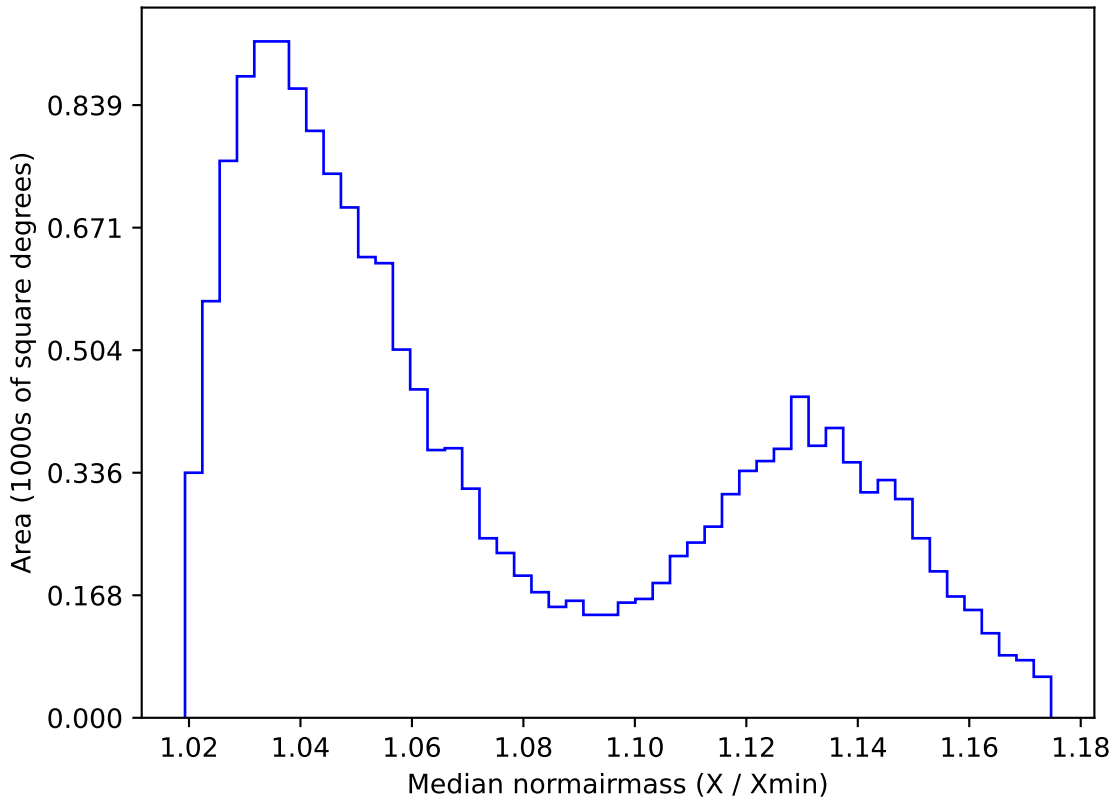
ddf_acor_sf20_lsf0_lsr0_v3.4_10yrs WFD i band: Median normairmass
