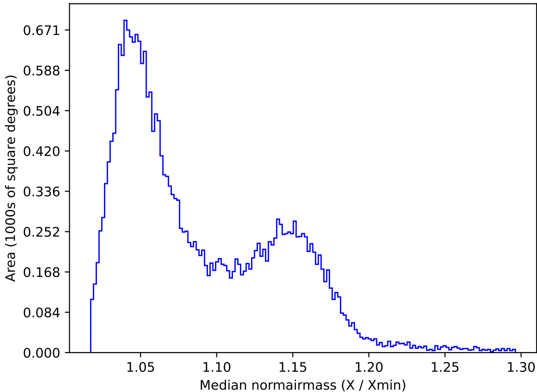
ddf_acor_sf20_lsf0_lsr0_v3.4_10yrs All sky z band: Median normairmass
