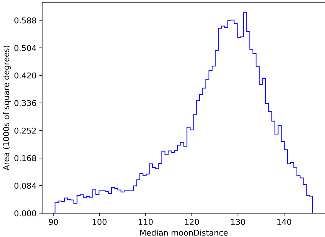
ddf_acor_sf20_lsf0_lsr0_v3.4_10yrs WFD u band: Median moonDistance
