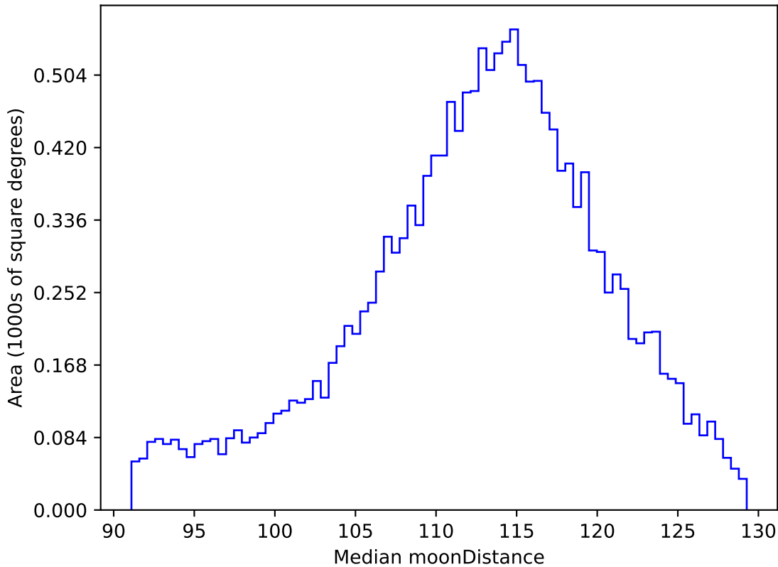
ddf_acor_sf20_lsf0_lsr0_v3.4_10yrs WFD r band: Median moonDistance
