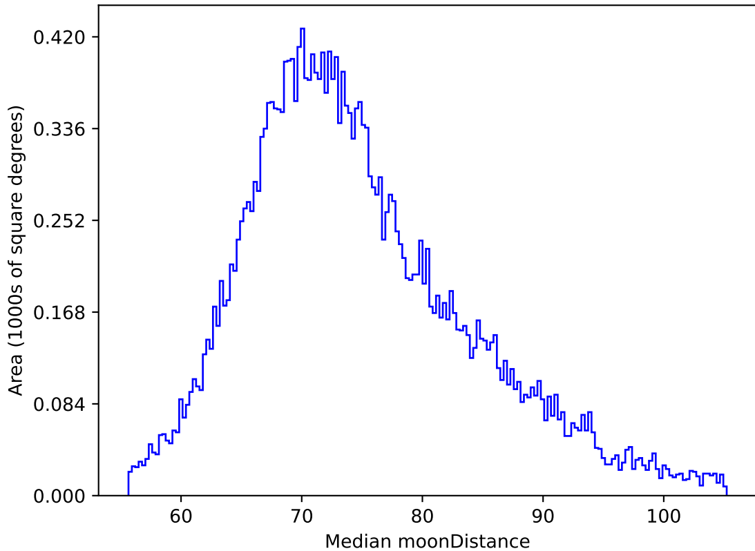
ddf_acor_sf20_lsf0_lsr0_v3.4_10yrs All sky z band: Median moonDistance
