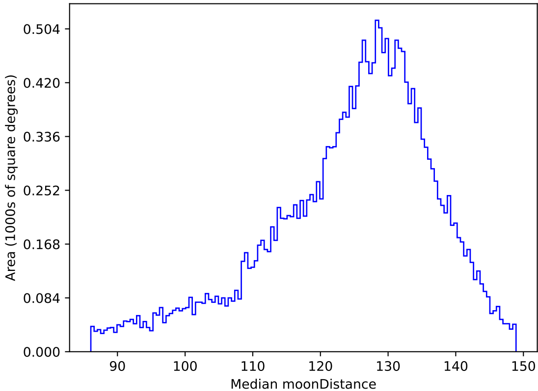
ddf_acor_sf20_lsf0_lsr0_v3.4_10yrs All sky u band: Median moonDistance
