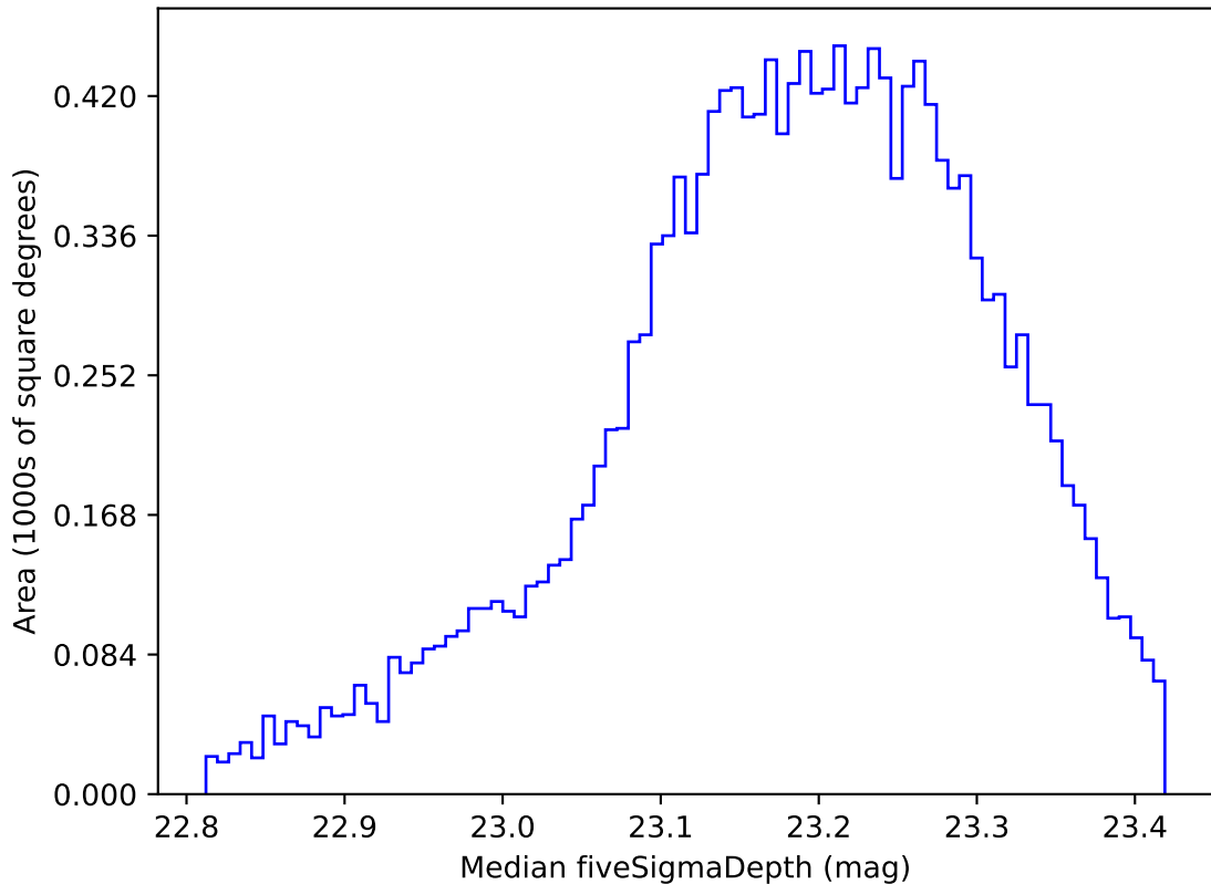
ddf_acor_sf20_lsf0_lsr0_v3.4_10yrs WFD u band: Median fiveSigmaDepth
