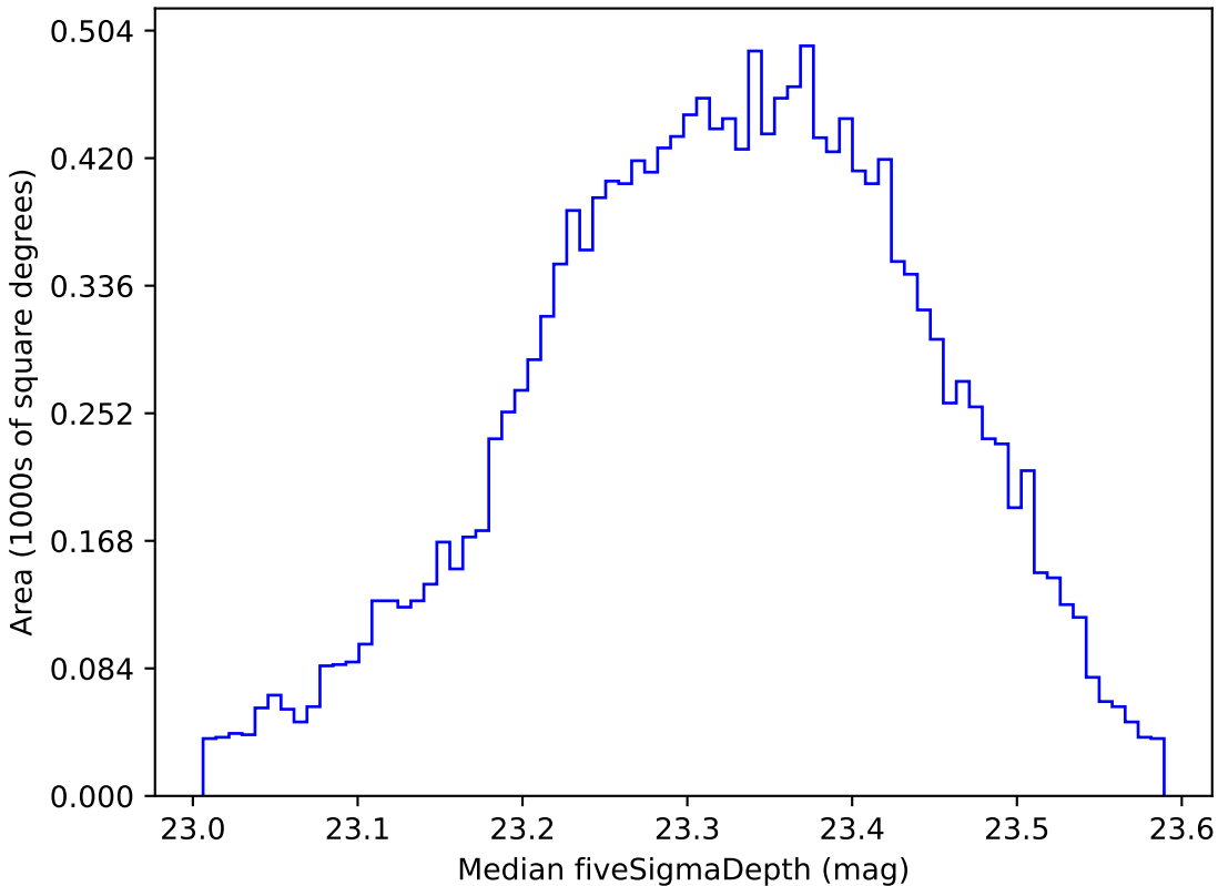
ddf_acor_sf20_lsf0_lsr0_v3.4_10yrs WFD all bands: Median fiveSigmaDepth
