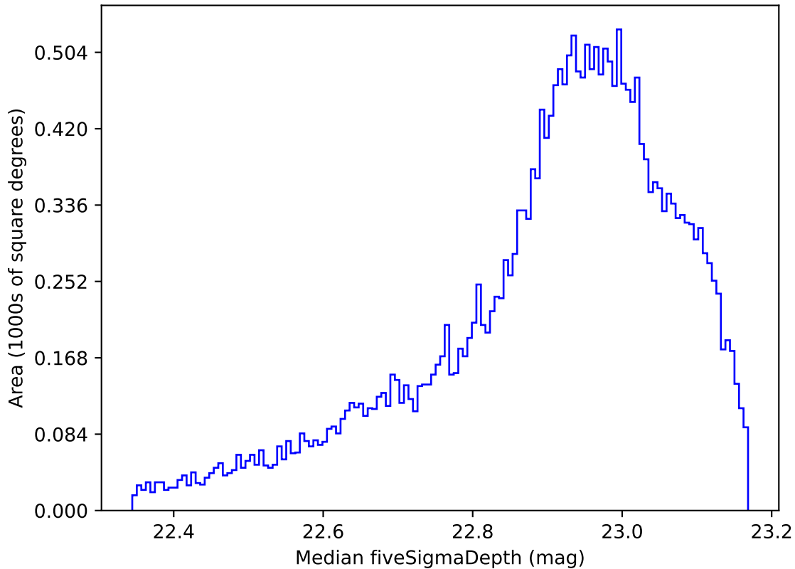
ddf_acor_sf20_lsf0_lsr0_v3.4_10yrs All sky z band: Median fiveSigmaDepth
