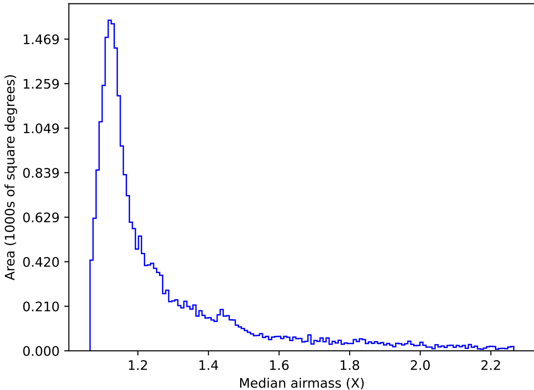
ddf_acor_sf20_lsf0_lsr0_v3.4_10yrs Yr 1 z band: Median airmass
