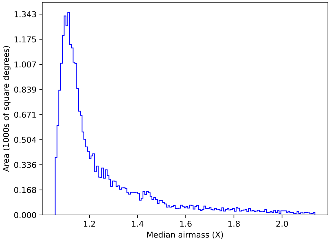
ddf_acor_sf20_lsf0_lsr0_v3.4_10yrs Yr 1 r band: Median airmass
