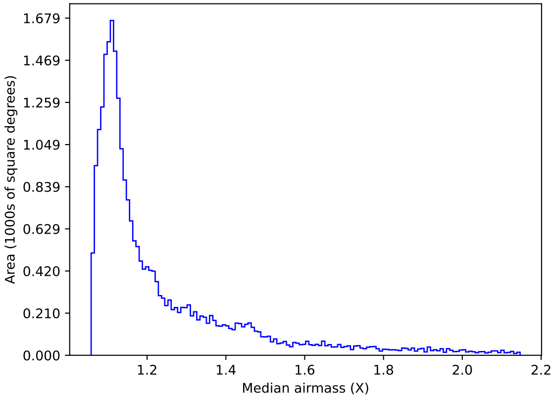
ddf_acor_sf20_lsf0_lsr0_v3.4_10yrs Yr 1 i band: Median airmass
