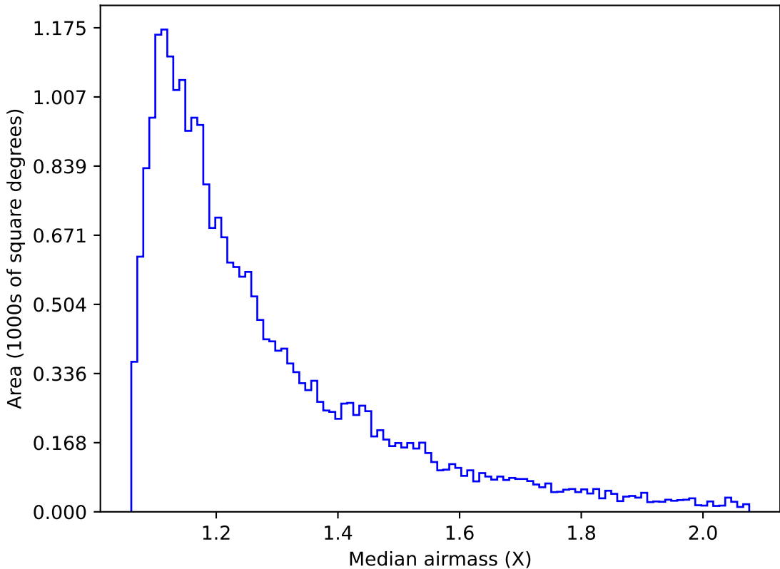
ddf_acor_sf20_lsf0_lsr0_v3.4_10yrs Yr 1 g band: Median airmass
