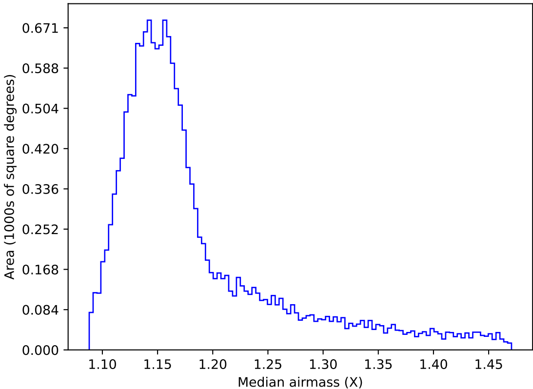
ddf_acor_sf20_lsf0_lsr0_v3.4_10yrs WFD z band: Median airmass
