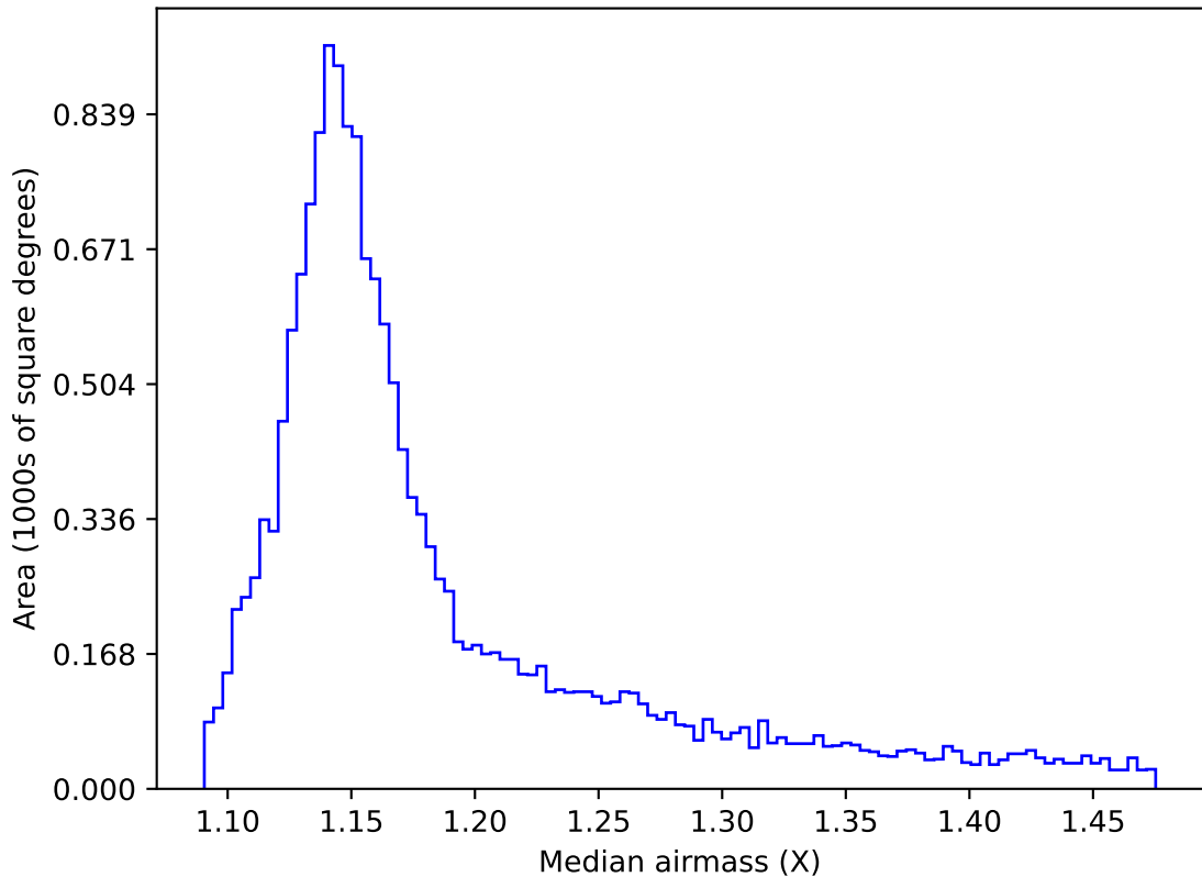
ddf_acor_sf20_lsf0_lsr0_v3.4_10yrs WFD y band: Median airmass
