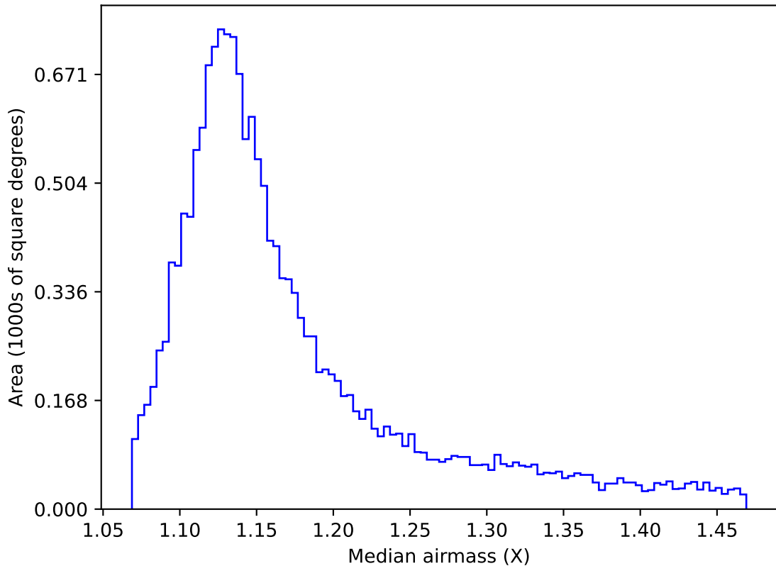
ddf_acor_sf20_lsf0_lsr0_v3.4_10yrs WFD u band: Median airmass
