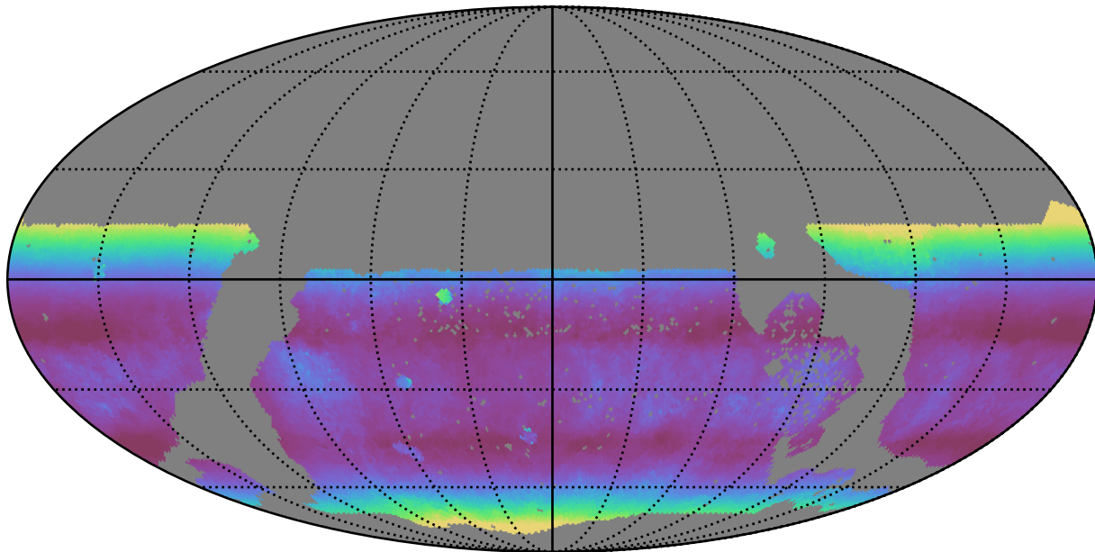
ddf_acor_sf20_lsf0_lsr0_v3.4_10yrs WFD r band: Median airmass
