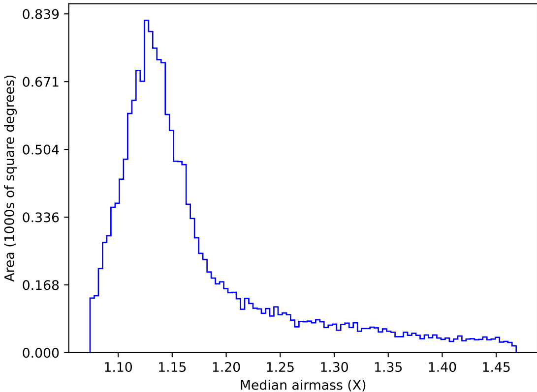
ddf_acor_sf20_lsf0_lsr0_v3.4_10yrs WFD r band: Median airmass
