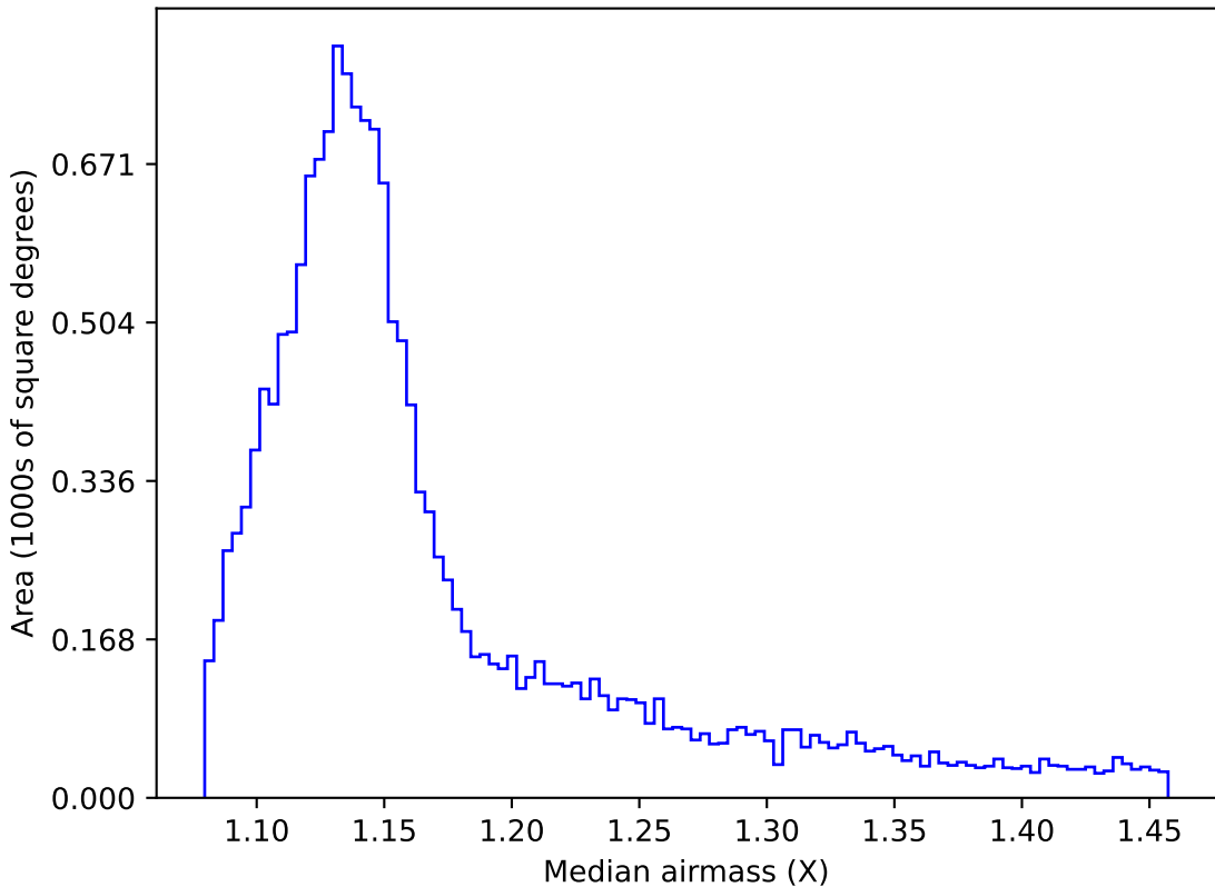
ddf_acor_sf20_lsf0_lsr0_v3.4_10yrs WFD i band: Median airmass
