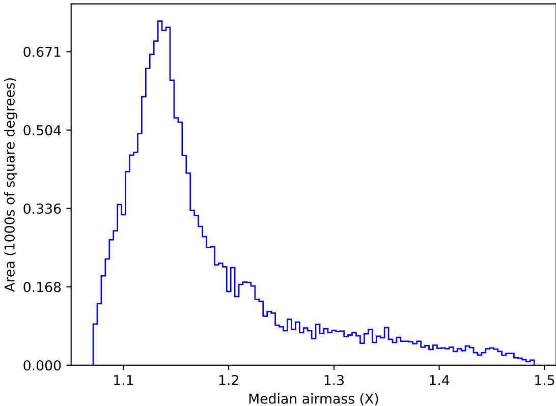
ddf_acor_sf20_lsf0_lsr0_v3.4_10yrs WFD g band: Median airmass
