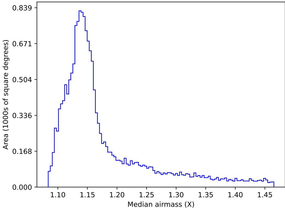
ddf_acor_sf20_lsf0_lsr0_v3.4_10yrs WFD all bands: Median airmass
