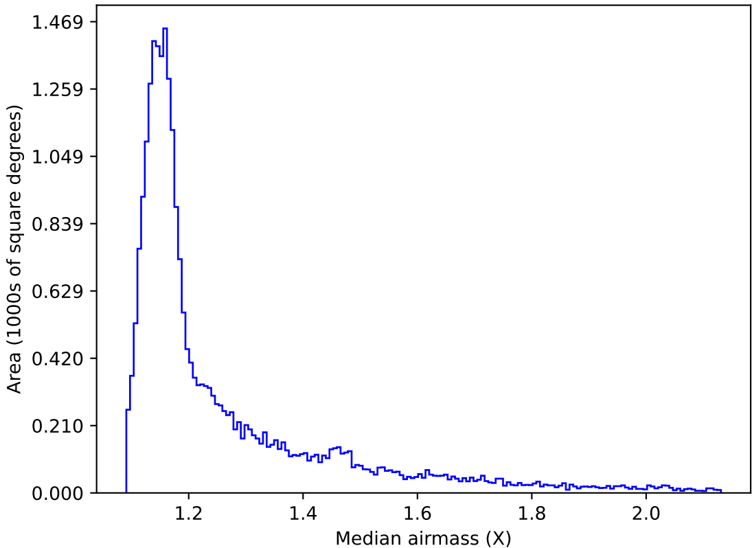
ddf_acor_sf20_lsf0_lsr0_v3.4_10yrs All sky z band: Median airmass
