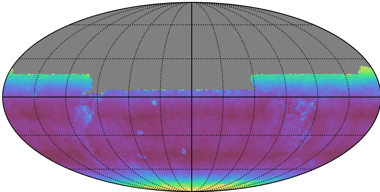
ddf_acor_sf20_lsf0_lsr0_v3.4_10yrs All sky y band: Median airmass
