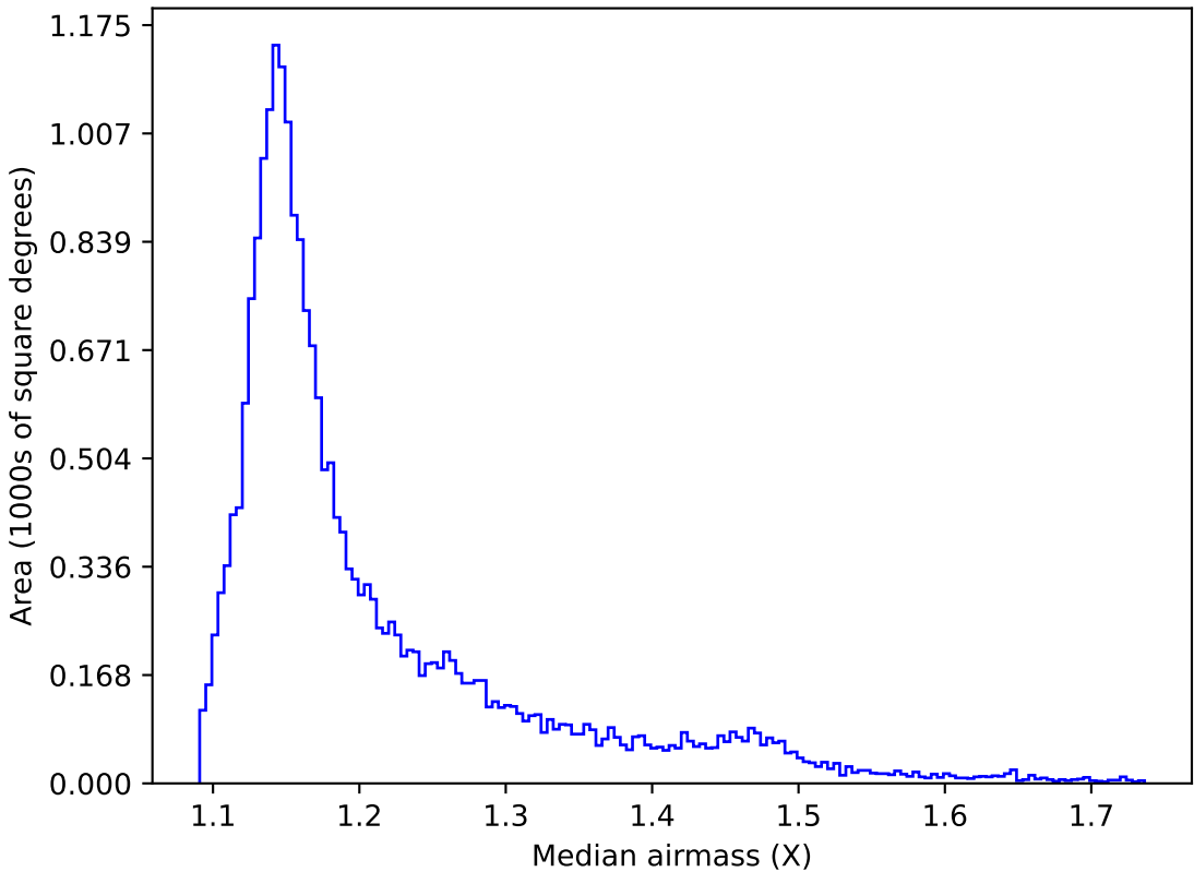
ddf_acor_sf20_lsf0_lsr0_v3.4_10yrs All sky y band: Median airmass
