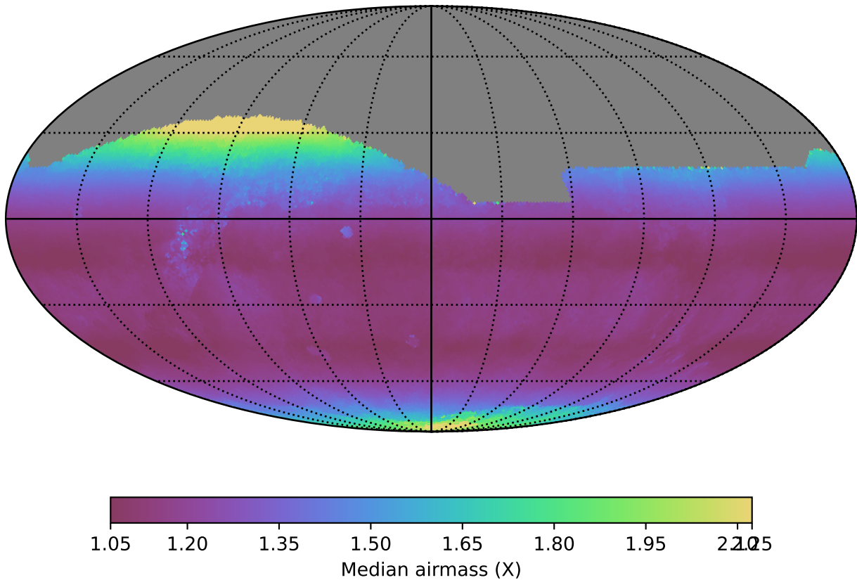
ddf_acor_sf20_lsf0_lsr0_v3.4_10yrs All sky r band: Median airmass
