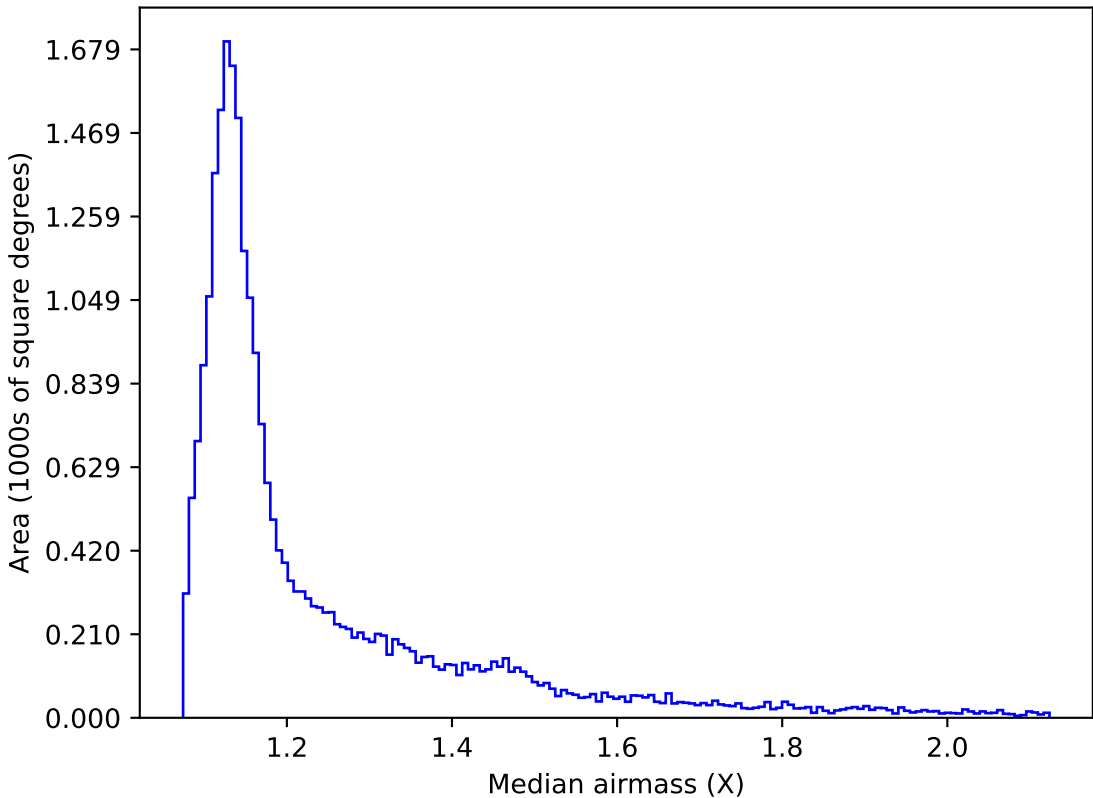
ddf_acor_sf20_lsf0_lsr0_v3.4_10yrs All sky r band: Median airmass
