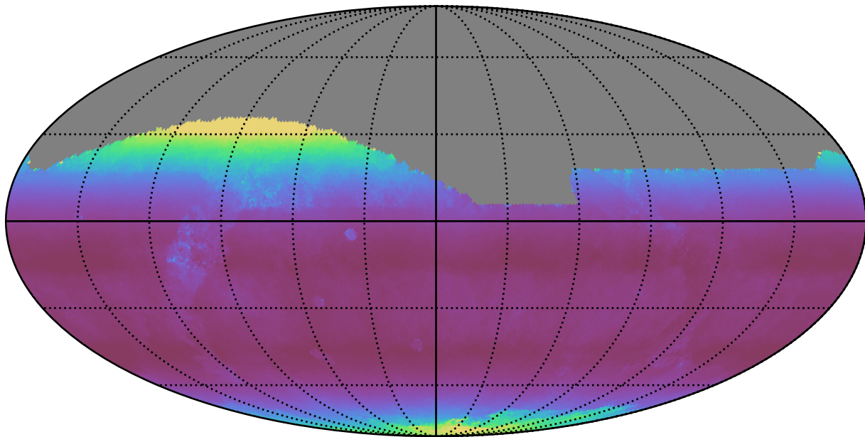
ddf_acor_sf20_lsf0_lsr0_v3.4_10yrs All sky i band: Median airmass
