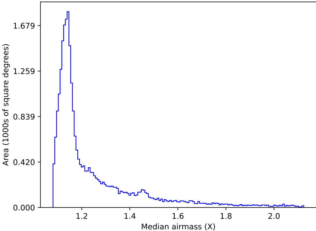
ddf_acor_sf20_lsf0_lsr0_v3.4_10yrs All sky i band: Median airmass
