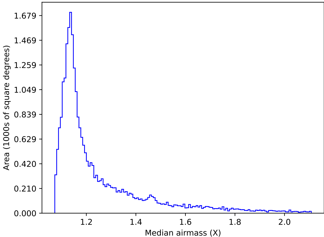
ddf_acor_sf20_lsf0_lsr0_v3.4_10yrs All sky g band: Median airmass
