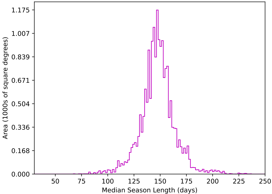
ddf_acor_sf20_lsf0_lsr0_v3.4_10yrs WFD z band: Median Season Length
