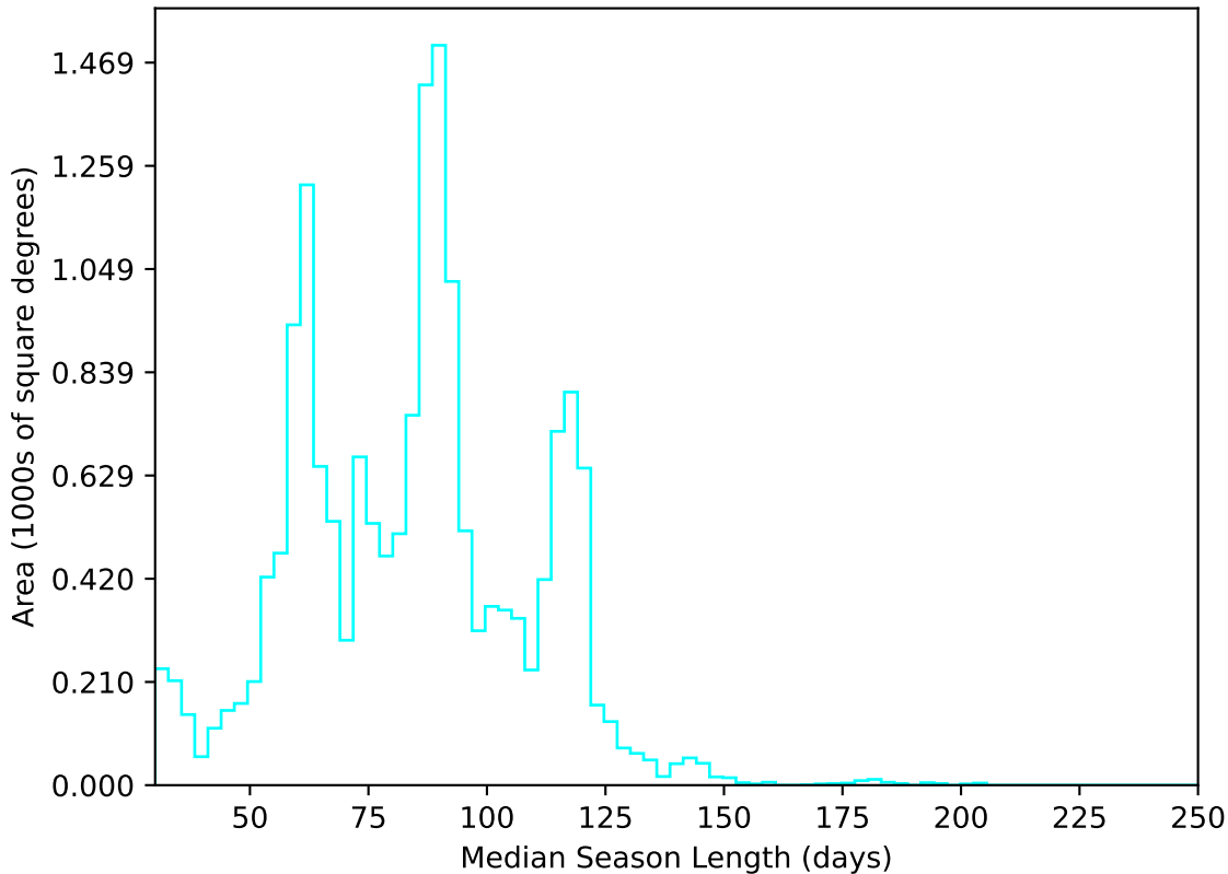
ddf_acor_sf20_lsf0_lsr0_v3.4_10yrs WFD u band: Median Season Length
