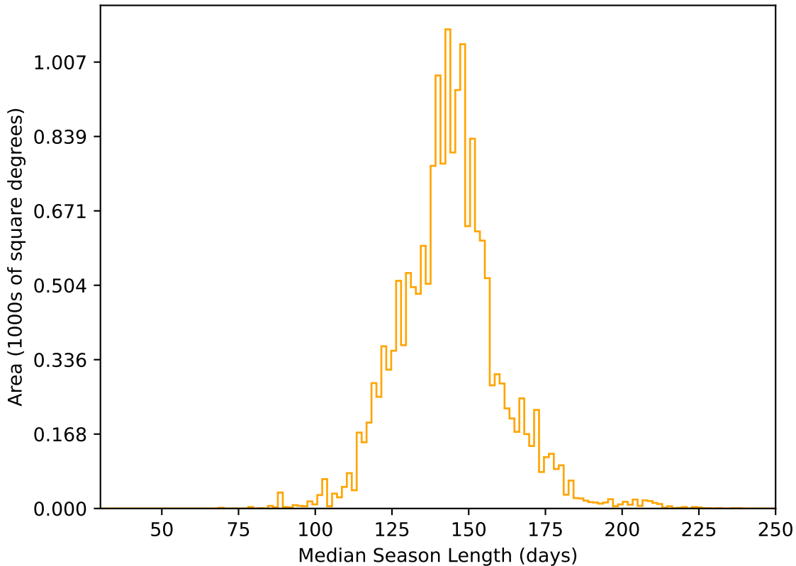
ddf_acor_sf20_lsf0_lsr0_v3.4_10yrs WFD r band: Median Season Length
