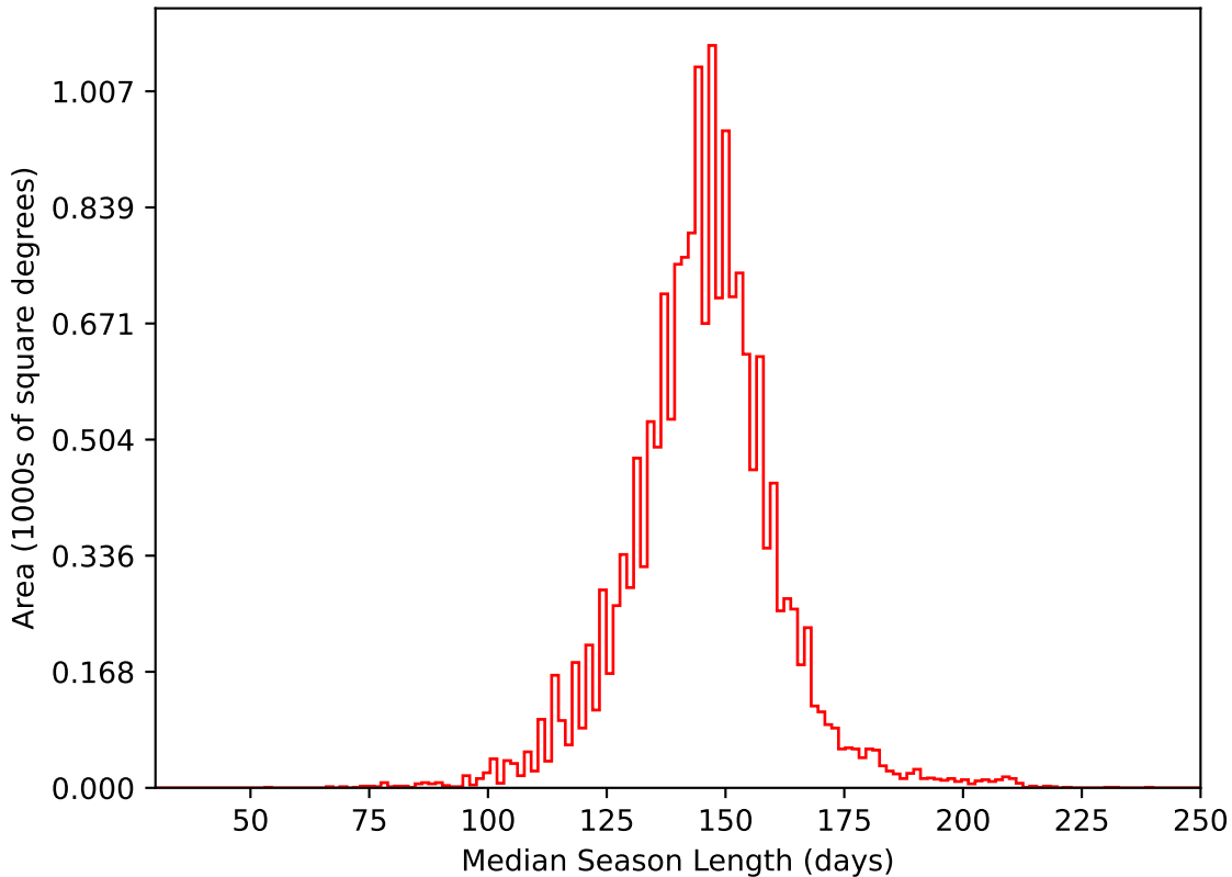
ddf_acor_sf20_lsf0_lsr0_v3.4_10yrs WFD i band: Median Season Length
