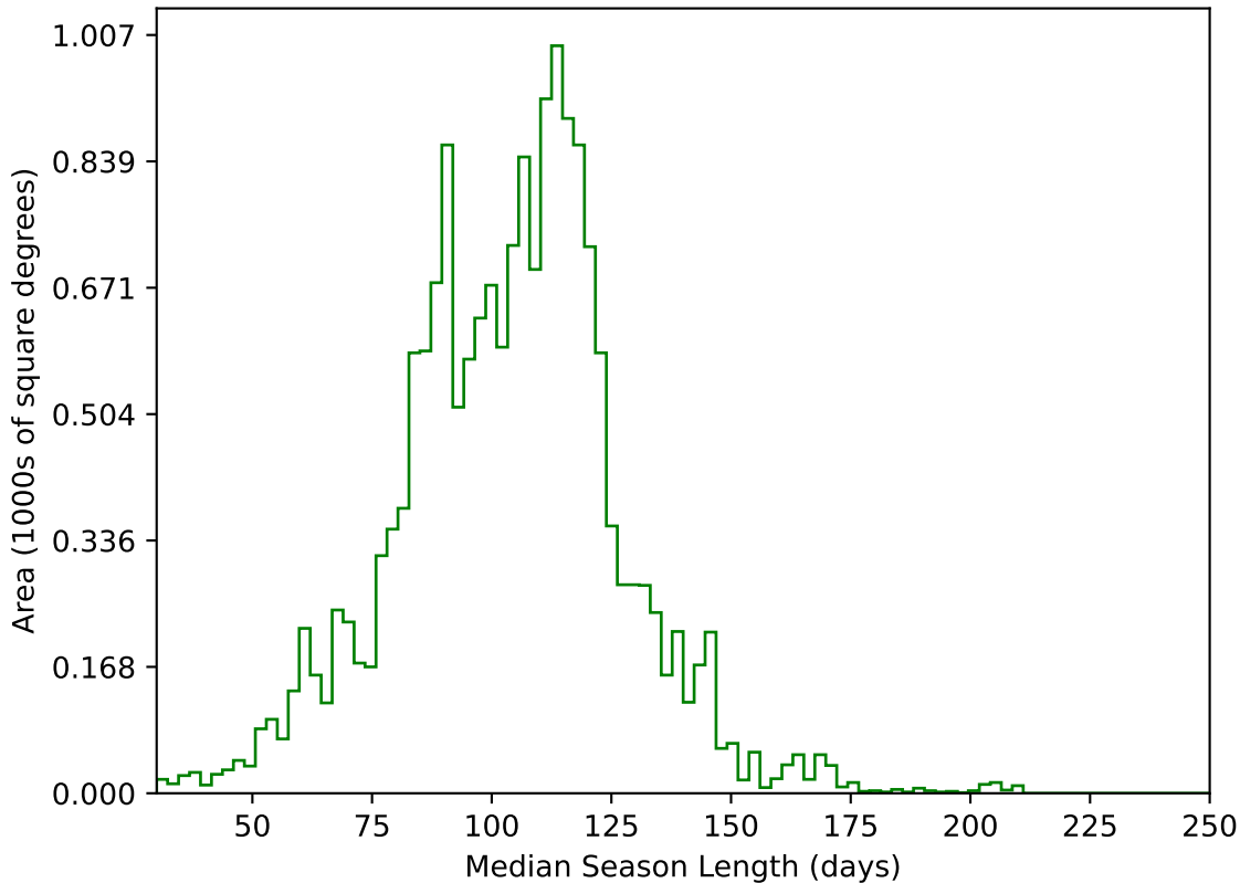
ddf_acor_sf20_lsf0_lsr0_v3.4_10yrs WFD g band: Median Season Length
