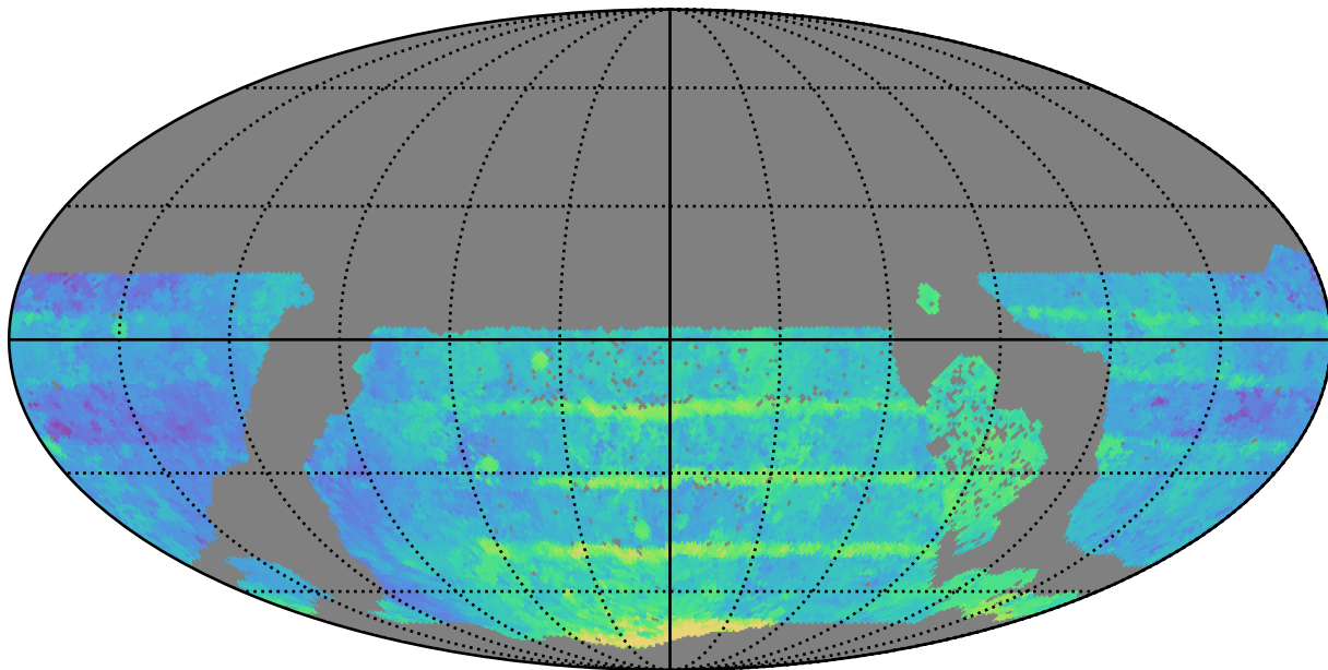
ddf_acor_sf20_lsf0_lsr0_v3.4_10yrs WFD all bands: Median Season Length
