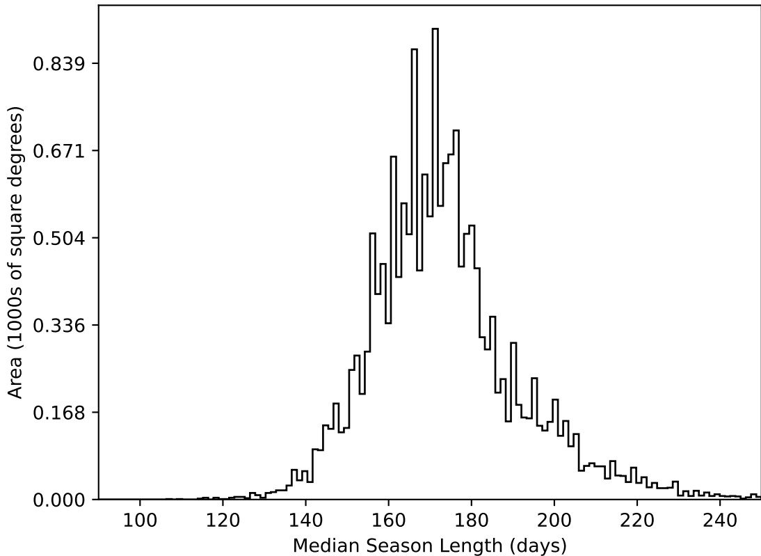
ddf_acor_sf20_lsf0_lsr0_v3.4_10yrs WFD all bands: Median Season Length
