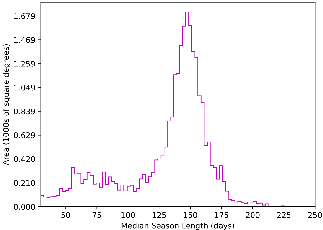
ddf_acor_sf20_lsf0_lsr0_v3.4_10yrs All sky z band: Median Season Length
