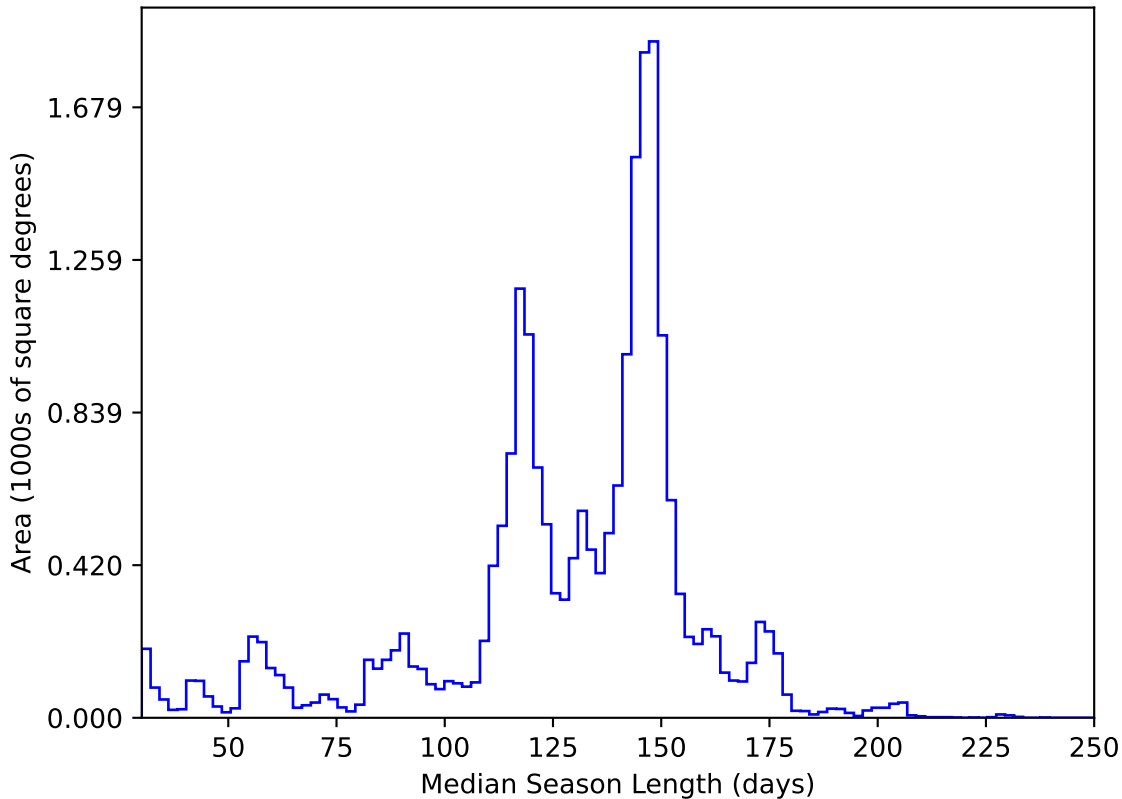
ddf_acor_sf20_lsf0_lsr0_v3.4_10yrs All sky y band: Median Season Length
