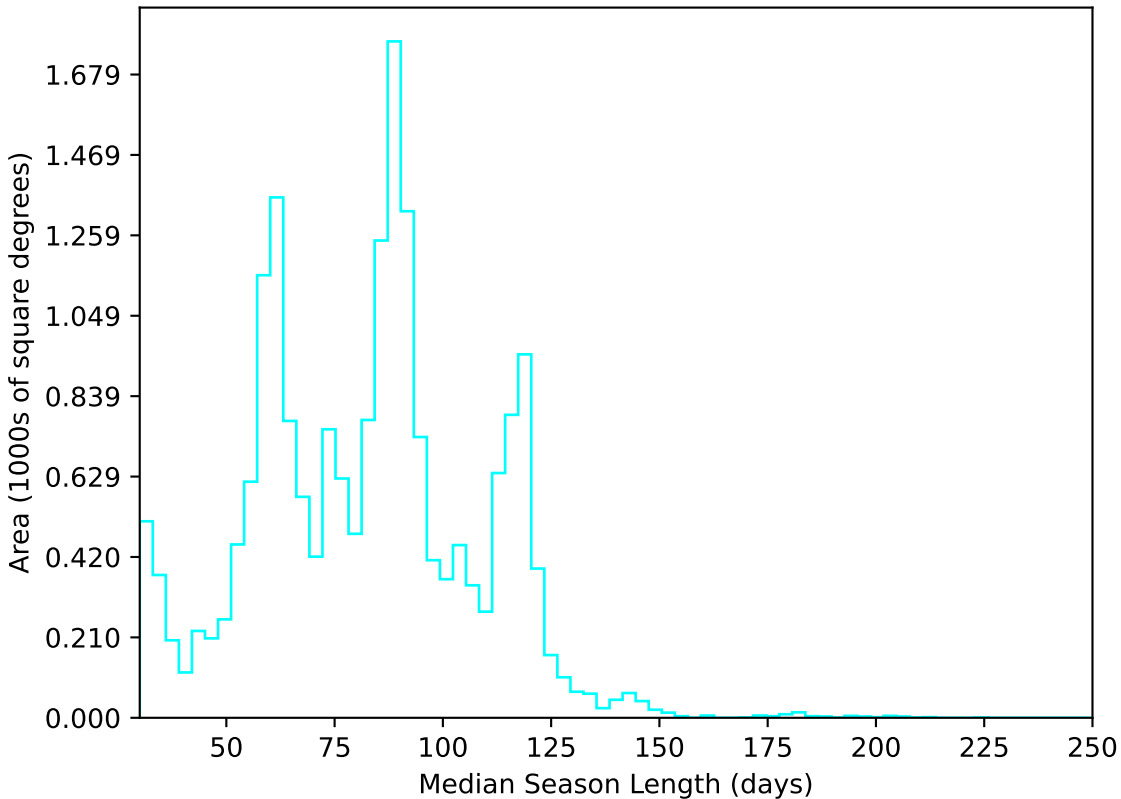
ddf_acor_sf20_lsf0_lsr0_v3.4_10yrs All sky u band: Median Season Length
