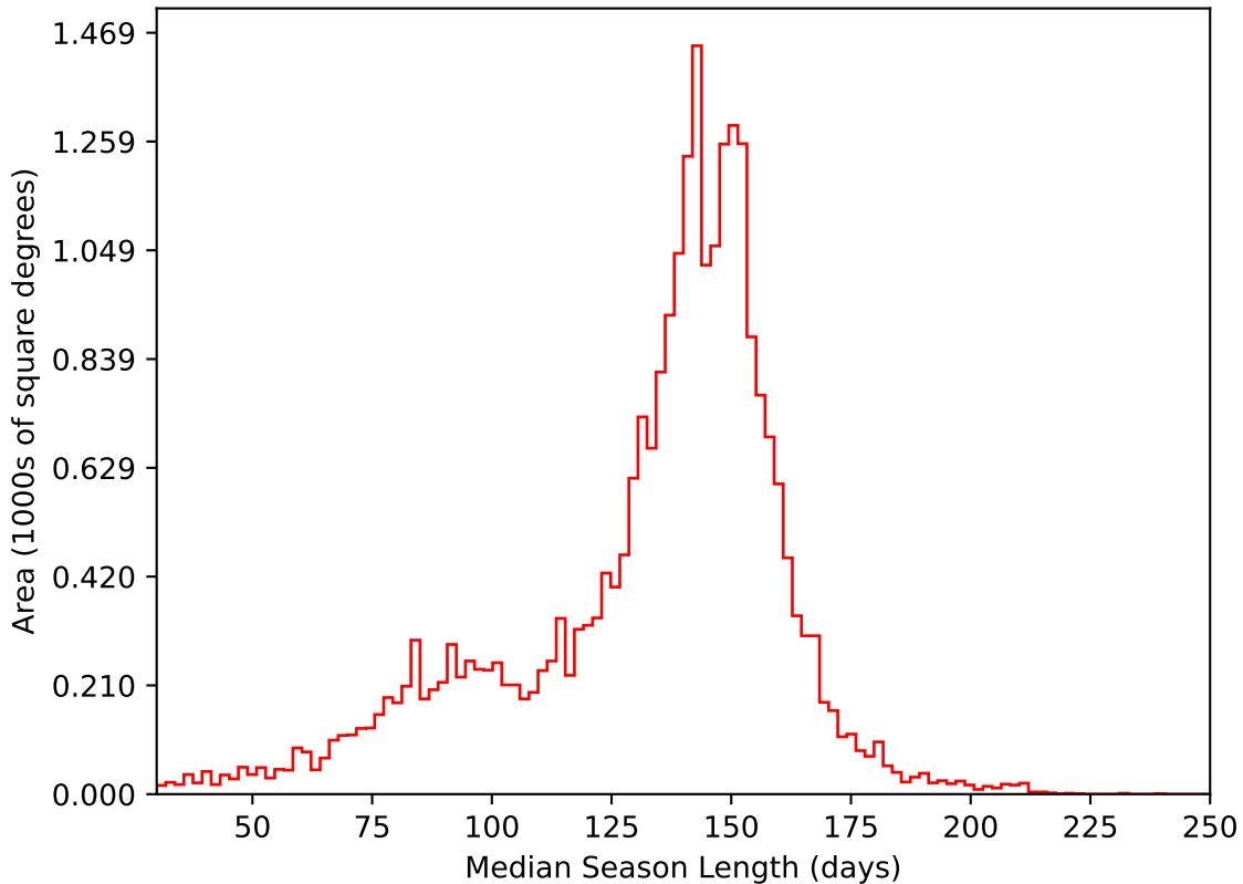
ddf_acor_sf20_lsf0_lsr0_v3.4_10yrs All sky i band: Median Season Length
