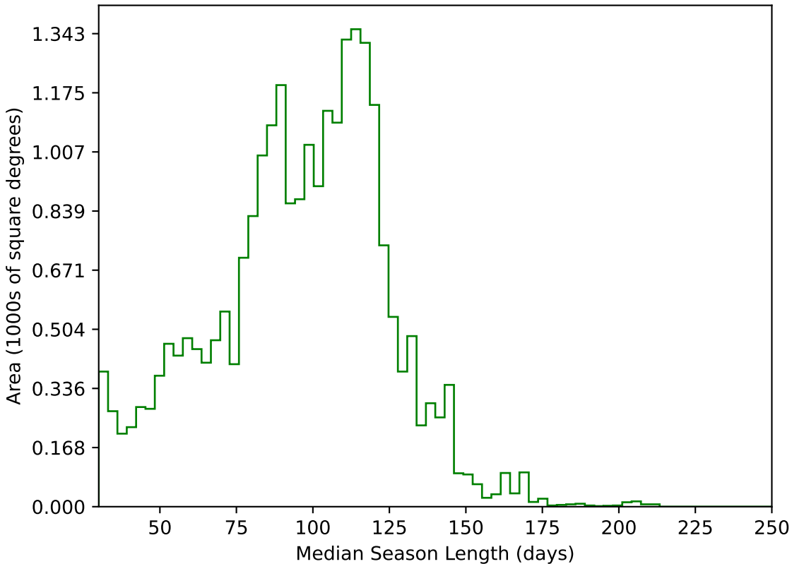
ddf_acor_sf20_lsf0_lsr0_v3.4_10yrs All sky g band: Median Season Length
