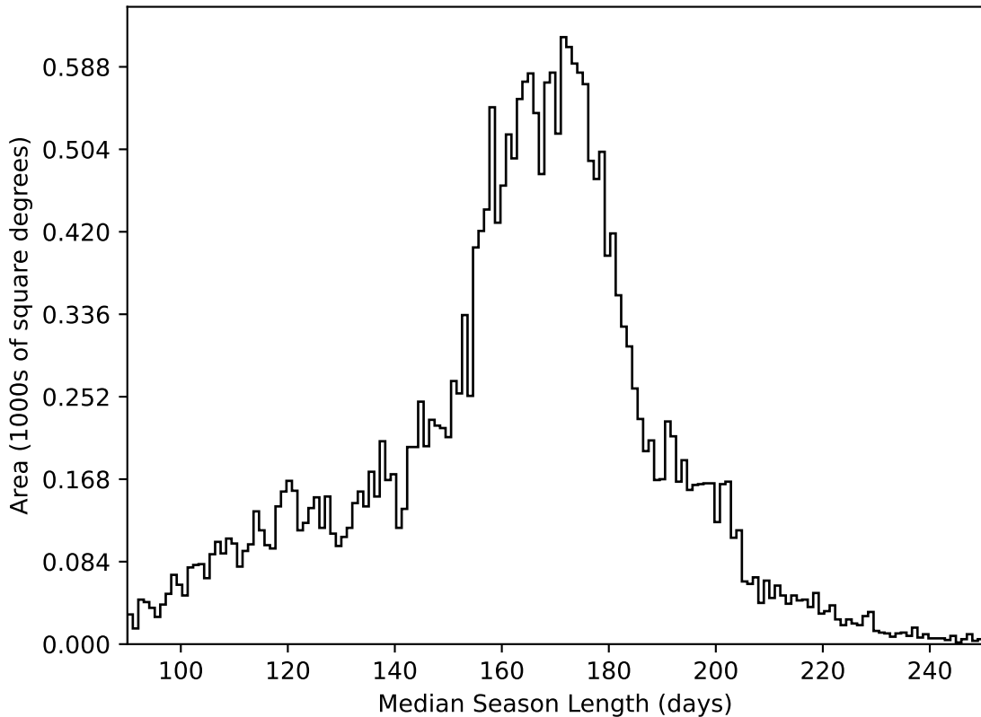
ddf_acor_sf20_lsf0_lsr0_v3.4_10yrs All sky all bands: Median Season Length
