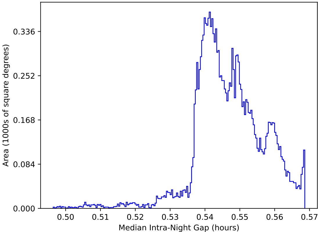
ddf_acor_sf20_lsf0_lsr0_v3.4_10yrs WFD: Median Intra-Night Gap
